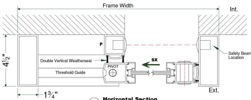
2 Horizontal Section Type P - SX
