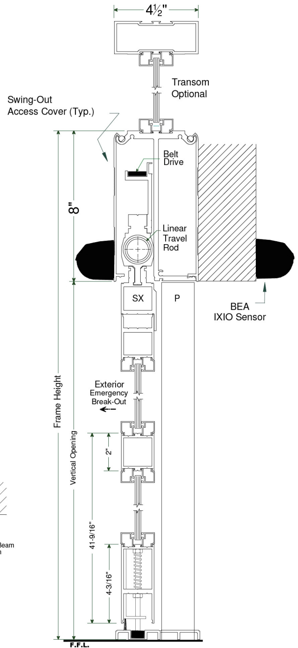
1 Vertical Section
